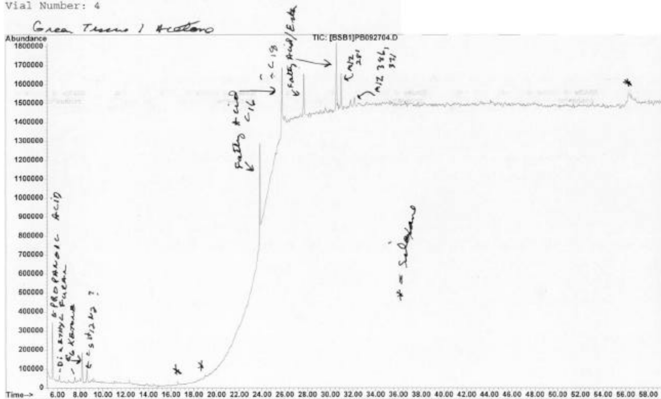
Figure 6. GC chromatogram of the acetone extract from the mutilated cow tissue (extraction #2).
