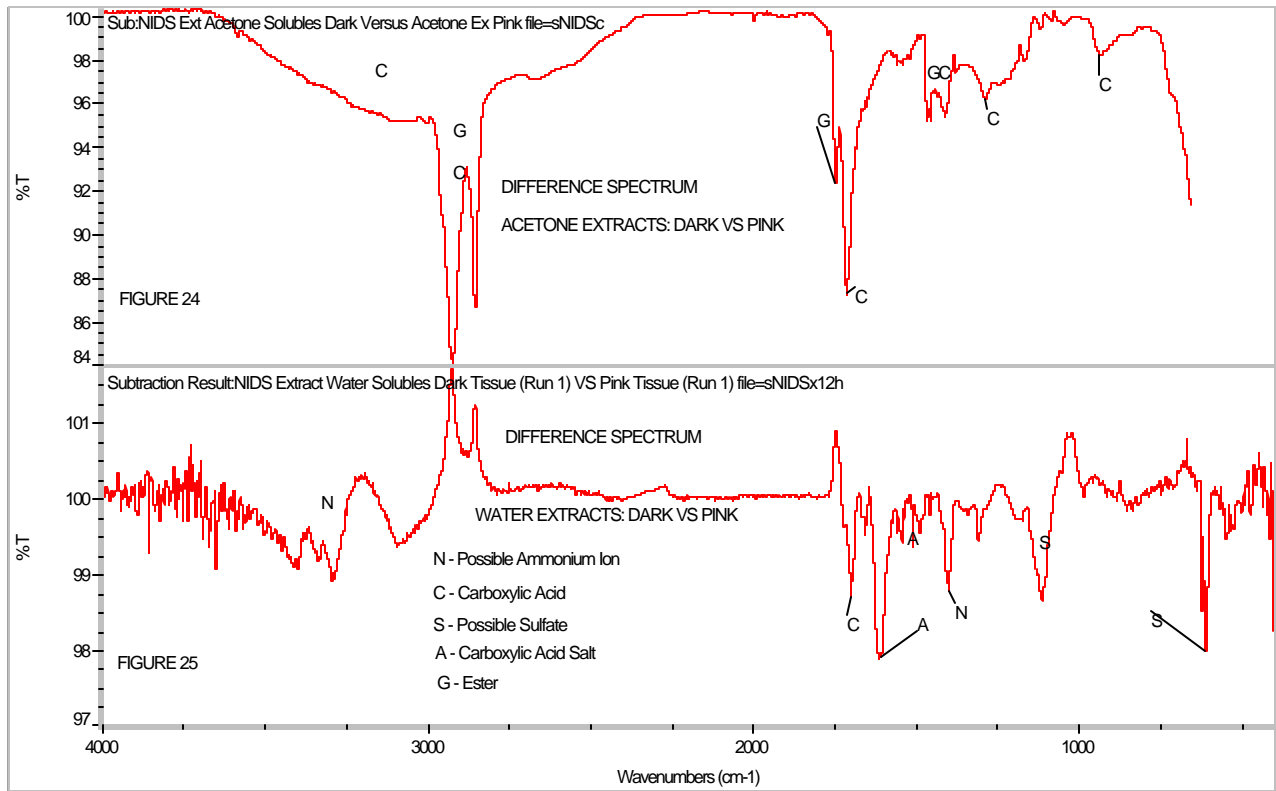
Figures 24, 25: Difference spectra of acetone and water extracts from the pink and dark tissues from the mutilated cow.
