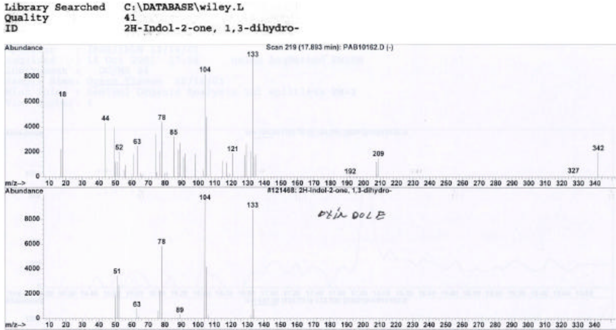
Figure 9. MS spectrum of oxindole from GC peak with retention time 17:54 min. of the chloroform extract from the mutilated cow (extraction #3) and oxindole reference.
