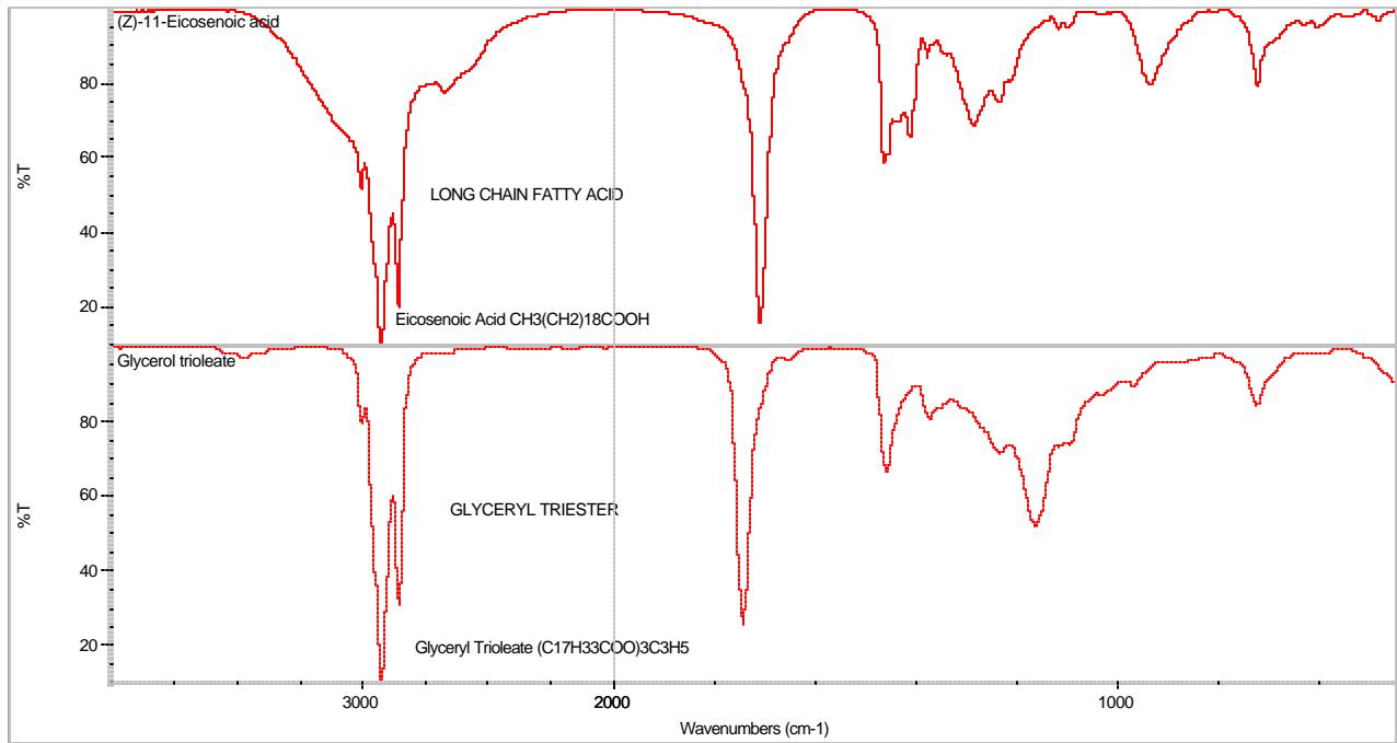
Figures 26, 27: Infrared reference spectra of a long chain fatty acid and a glyceryl triester.
